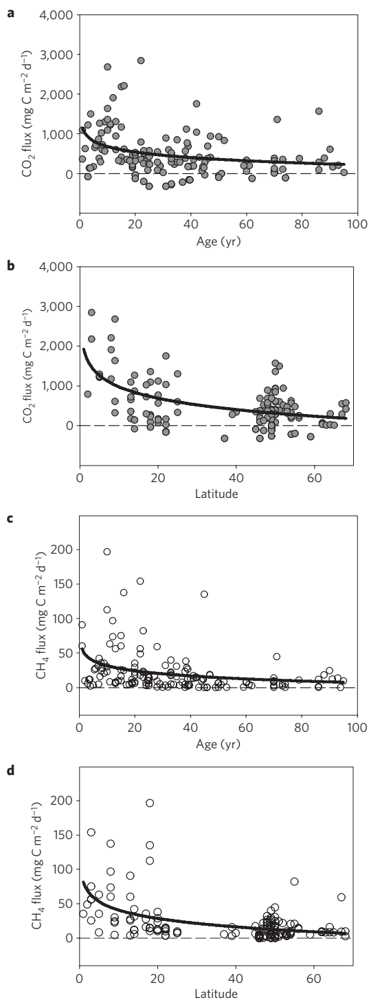
Figure 1 | Scatter plot and exponential decline for the relationships between CO 2 and CH 4 and age and latitude. a , CO 2 versus age (adjusted R^2 , Adj R^2 = 0.31 ; degrees of freedom (df) = 136; significance probabilities ( p ) < 0.0001). b , CO 2 versus latitude (Adj R^2 = 0.16 ; df = 120; p < 0.0001). c , CH 4 versus age (Adj R^2 = 0.39 ; df = 149; p < 0.0001) and d , CH 4 versus latitude (Adj R^2 = 0.17 ; df = 144; p < 0.0001).
