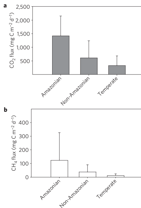
Figure 2 | Fluxes of CO 2 and CH 4 in different zones. Mean (bars) and standard deviation (lines) of the a , CO 2 and b , CH 4 fluxes in the 85 hydroelectric reservoirs worldwide distributed clustered by region. The tropical region was split into Amazonian and non-Amazonian regions.
